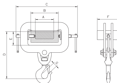
TZH, swivel hooks, pivoting and swivelling
